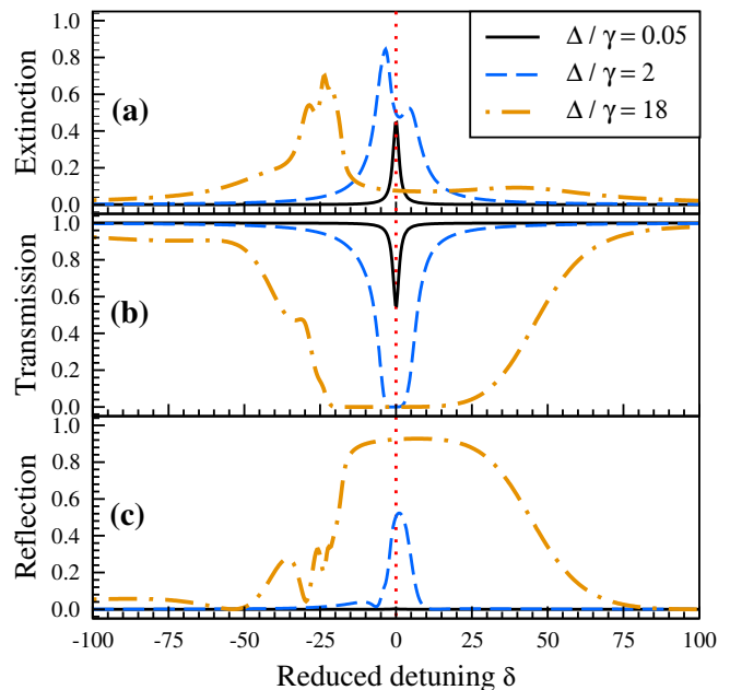
FIG. 2. (Color online) Extinction (a), transmission (b) and reflection (c) probabilities as a function of the reduced detuning \delta = (\omega - \omega_{01})/\gamma for a layer thickness \ell = \lambda_0/1.55 = 400 nm. The decay and pure dephasing rates are 10^{11} Hz and 10^{12} Hz. The solid black lines correspond to a weak density where \Delta/\gamma = 0.05 , the dashed blue lines are for an average density with \Delta/\gamma = 2 , and the dash-dotted brown lines stand for a large density where \Delta/\gamma = 18 .
