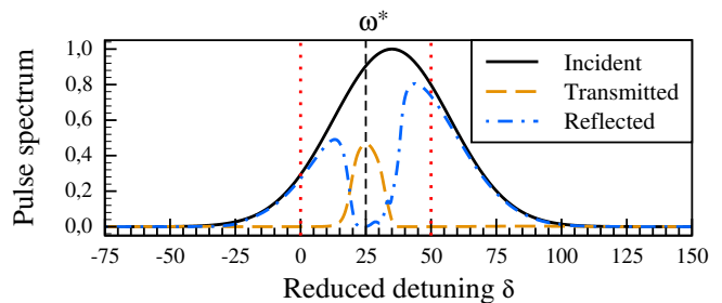
FIG. 5. (Color online) Incident (solid black line), transmitted (dashed brown line) and reflected (dash-dotted blue line) pulse spectrum in the case of a dense vapor constituted by a mixture of two different quantum emitters, for large densities. All parameters are as in Fig. 4.
