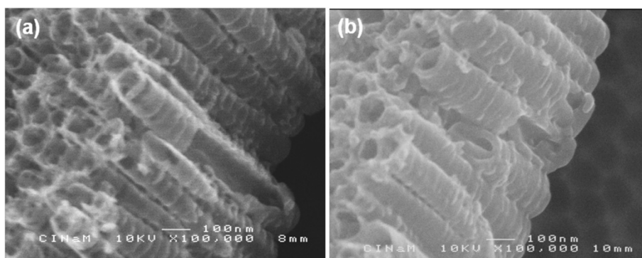
Figure 3 Cross-sectional images of the copolymer-embedded TiO 2 nt after (a) 1 cycle and (b) 10 cycles.
