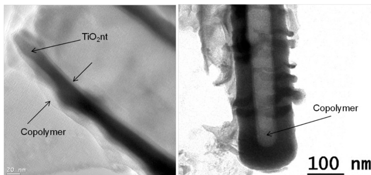
Figure 4 TEM images of copolymer-embedded TiO 2 nt after 5 cycles of CV. (a) Deposition of a homogeneous copolymer layer onto the inner and outer walls of the nanotube and (b) examination of the bottom part of the tube.
