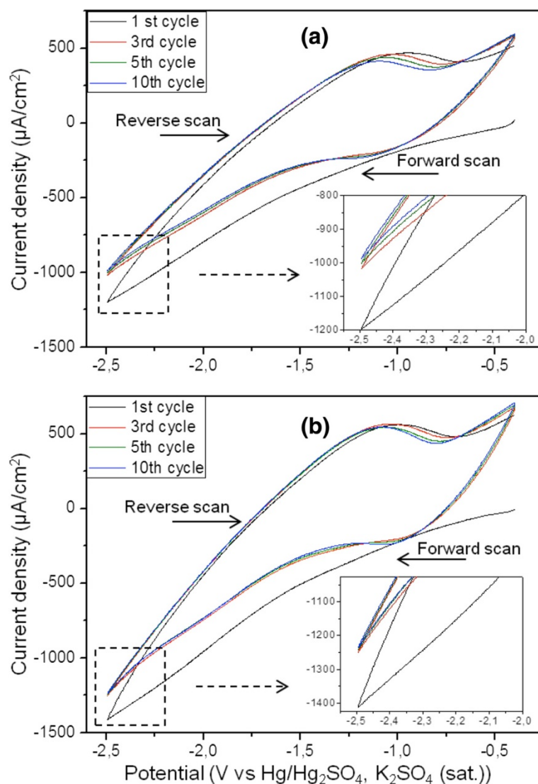
Figure 1 Cyclic voltammograms of TiO 2 nt electrode. In (a) 0.035 M LiTFSI and (b) in 0.035 M LiTFSI + 4 g MMA-PEO at the 1st, 3rd, 5th, and 10th cycles. The electropolymerization was carried out between -0.4 and -2.5 V vs Hg/Hg 2 SO 4 , K 2 SO 4 (saturated) with the scan rate of 25 mV/s.
