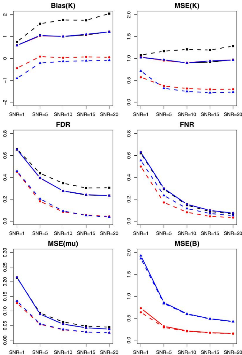
Fig. 2. Estimation performance in terms of bias and MSE according to SNR, calling, and normalization when using CBS. Dashed line: without calling, solid line: with calling, \blacksquare without normalization, \bullet (red) with position effect correction, and \blacktriangle (blue) spline-based normalization.
