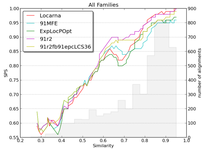
Fig. 5. SPS value for all 5 methods applied to the Bralibase2.1 benchmark.
