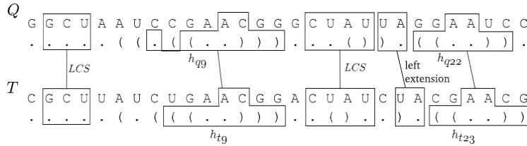
Fig. 3. The matches between Q and T are left extended only for h_{q22} and h_{t23} and gaps are filled thanks to LCS computation.
