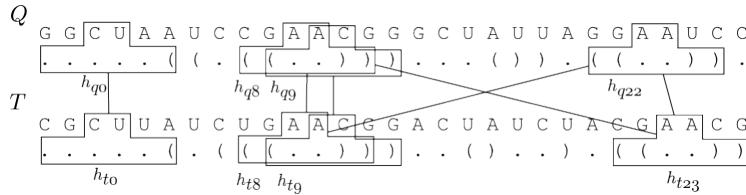
Fig. 1. Example of hits between two RNAs Q and T . We can notice that h_{q8} / h_{q9} and h_{t8} / h_{t9} are overlapping hits and h_{q8} / h_{t23} and h_{t8} / h_{q22} are crossing hits. So there is 6 hits \{(h_{q0}; h_{t0}), (h_{q8}; h_{t8}), (h_{q8}; h_{t23}), (h_{q22}; h_{t8}), (h_{q9}; h_{t9}), (h_{q22}; h_{t23})\} .
