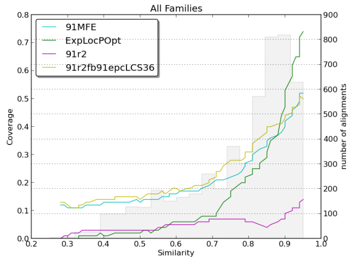
Fig. 6. Coverage of RNA sequences by anchors in percent for all 4 seeds-based methods ( LocaRNA alone does not use seeds) applied to the Bralibase2.1 benchmark.
