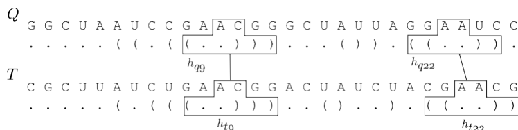
Fig. 2. Compared to Fig. 1 3 hits are lost because of structural composition, crossing and overlapping. So this example show the final hits between Q and T .
