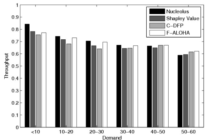
(b) 50 nodes
