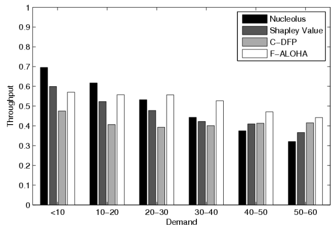
(c) 100 nodes
