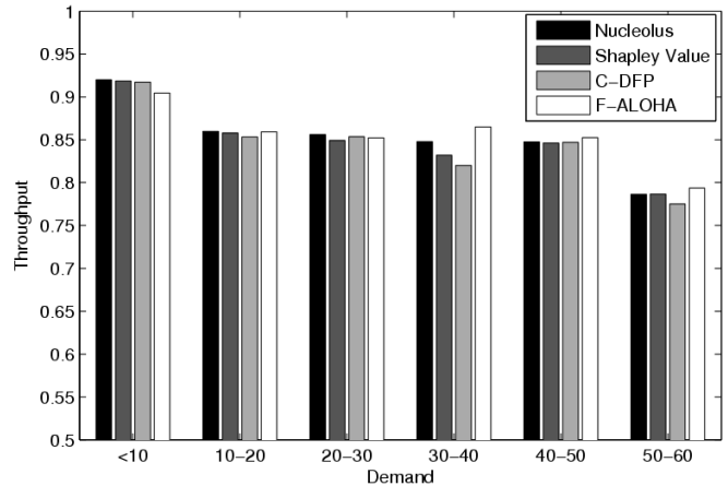
(a) 25 nodes
