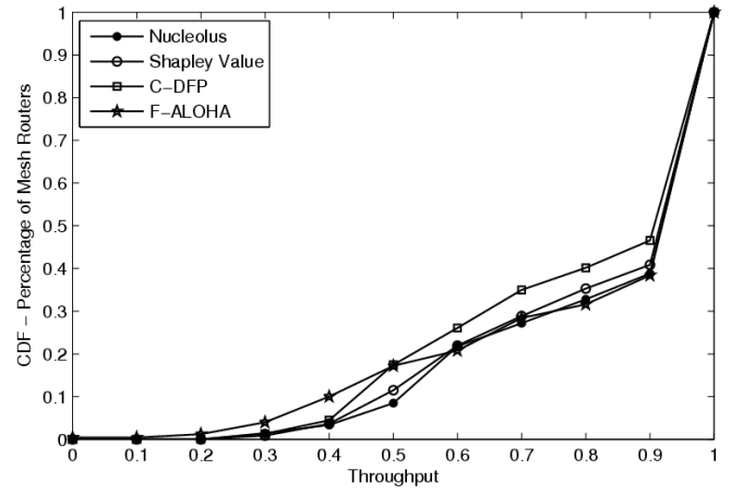
(a) 25 nodes
