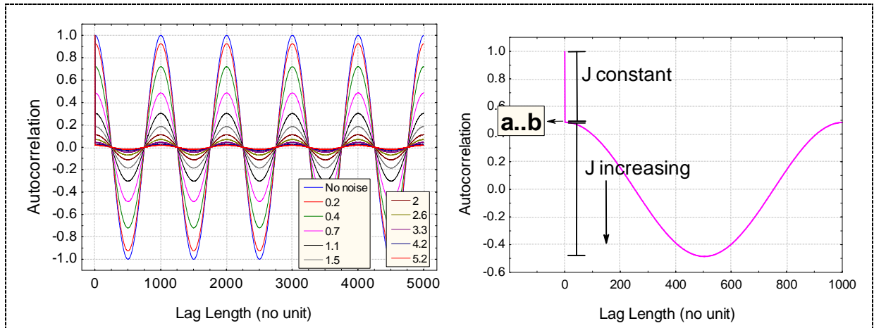
Figure 2. Autocorrelation function of sinus functions test with white noise at different amplitude level (left) and an zoom of Autocorrelation function of a noisy sinus function (right) with notations used in the text.
