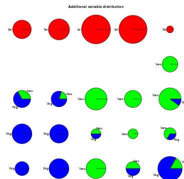
Fig. 2. Pie charts of Species for a SOM trained on the four numeric variables of the iris dataset.
