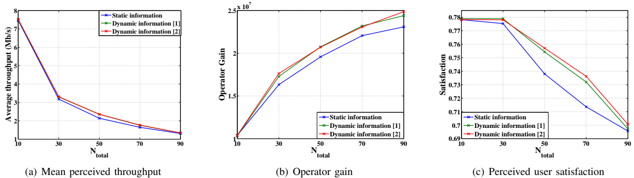
Fig. 7. Operator gain and global network performance
