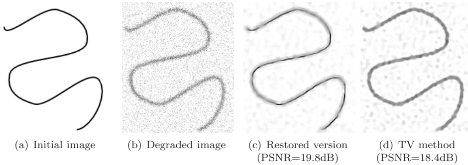
FIG. 16. Comparison of the restoration (5.3) ( \beta = 1 ) with the TV model for a Gaussian blurred ( \sigma = 1.5 ) and Gaussian noisy (PSNR=15.7dB) synthetic image
