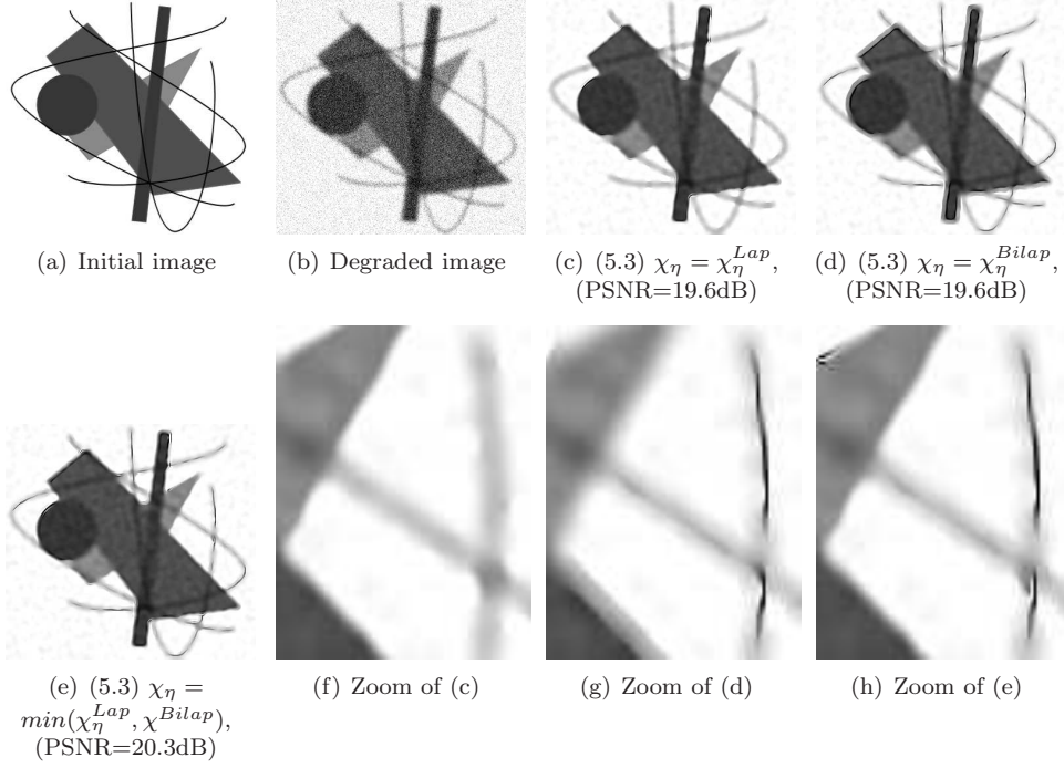
FIG. 20. Comparison of the restoration process (5.3) ( \beta = 2 ) with different choices of function \chi_\eta for a Gaussian blurred and noisy image ( \sigma = 3 , PSNR=15.7dB)
