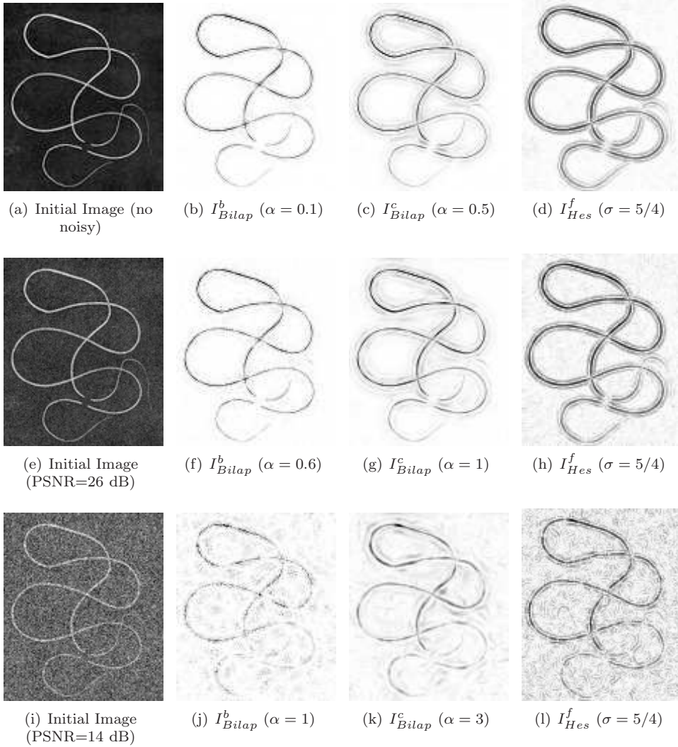
FIG. 8. Study of the robustness with respect to noise of I_{Bilap}^b (4.3a), I_{Bilap}^c (4.3b) and I_{Hes}^f (6.1) on a synthetic image. Each row matches a level of noise and each column is associated to an indicator.
