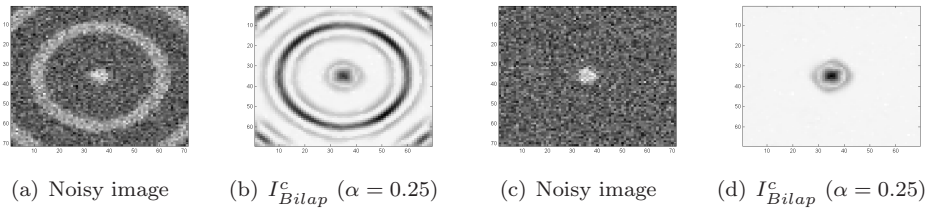
FIG. 24. A 2D cut ( z = z_c ) of I_{Bilap}^c (11.1) for two Gaussian noisy images (PSNR=16dB).
