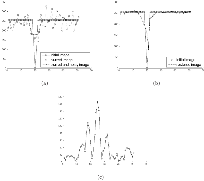
FIG. 19. (a) A transverse cut displaying the motion blurring ( \theta = 90^\circ , length=7) and the Gaussian noise effects (PSNR=15.7dB), (b) the initial image and the restored version (5.3) ( \gamma = 1 ) and (c) I_{Bilap}^c for \alpha = 0.7
