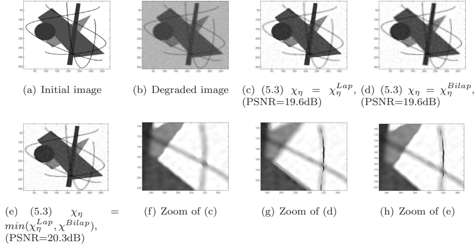
FIG. 20. Comparison of the restoration process (5.3) ( \beta = 2 ) with different choices of function \chi_\eta for a Gaussian blurred and noisy image ( \sigma = 3 , PSNR=15.7dB)
