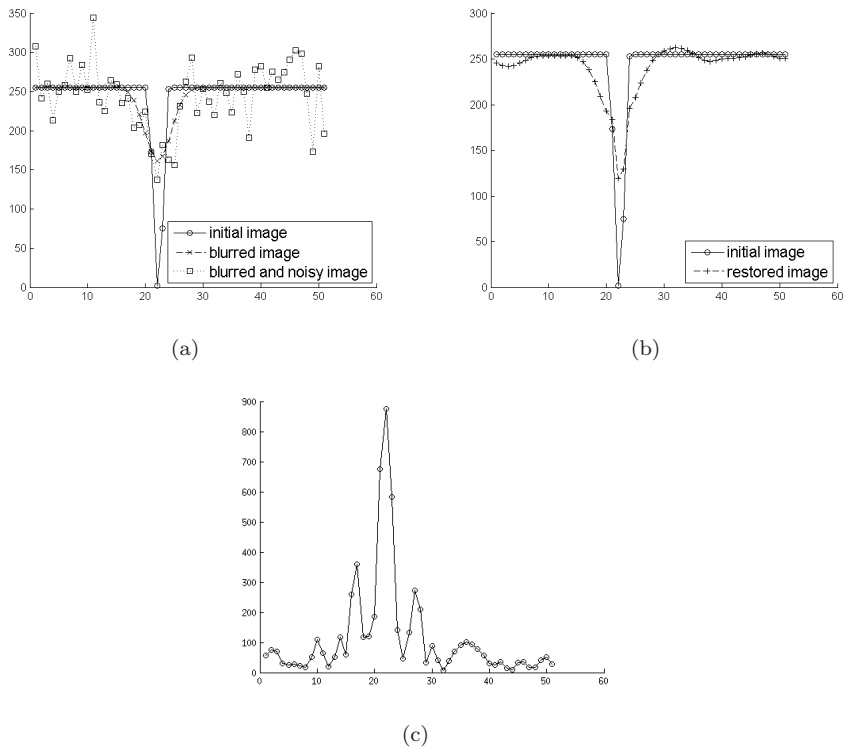
FIG. 18. (a) A transverse cut displaying the Gaussian blurring ( \sigma = 2.1 ) and the Gaussian noise effects ( PSNR=15.7dB ), (b) the initial image and the restored version (5.3) ( \beta = 1 ) and (c) I_{Bilap}^c (4.3b) for \alpha = 0.1
