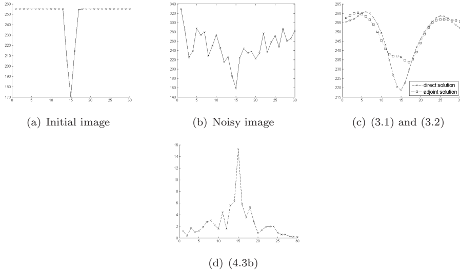
FIG. 7. A transverse cut displaying (a) the initial image, (b) its noisy version (PSNR=26dB), (c) the direct and adjoint solutions and (d) I_{Bilap}^c for \alpha = 0.8
