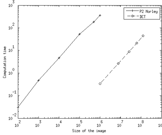
FIG. 4. Variation of the u_0 and v_0 computational time for u_0 and v_0 according to the size of the image using the logarithmic scale for both DCT and P2-Morley methods.
