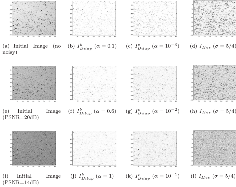
FIG. 13. Study of the robustness with respect to noise of I_{Bilap}^b (4.3a), I_{Bilap}^c (4.3b) and I_{Hes}^p (6.1) on a real non noisy image and on its noisy versions. Each row matches a level of noise and each column is associated to an indicator
