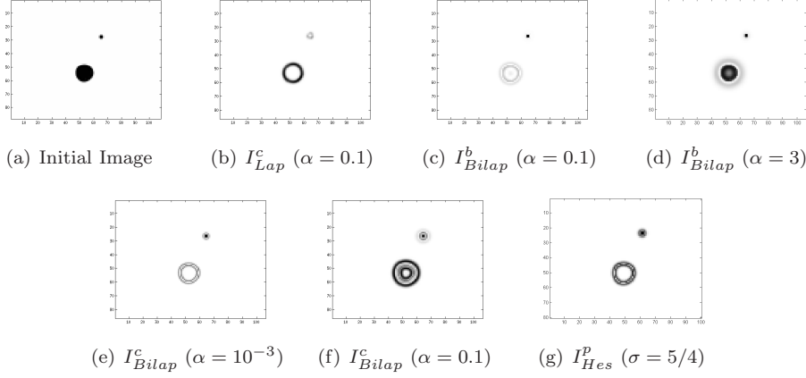
FIG. 10. Comparison of I_{Lap}^c (5.1), I_{Bilap}^b (4.3a), I_{Bilap}^c (4.3b) and I_{hes}^p (6.1) on a simple synthetic image without noise
