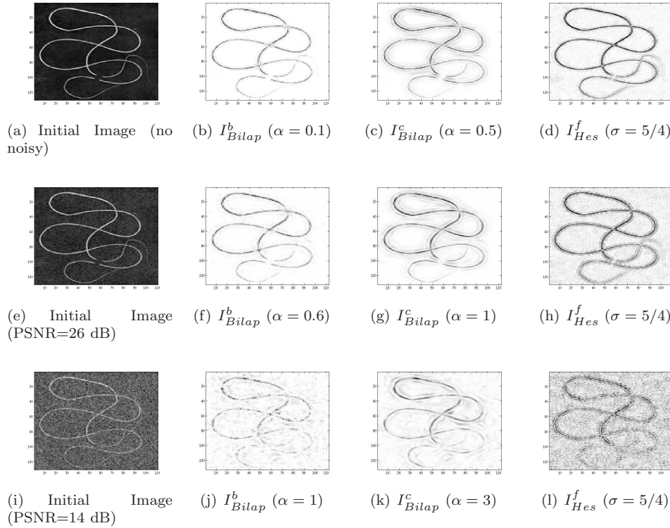
FIG. 8. Study of the robustness with respect to noise of I_{Bilap}^b (4.3a), I_{Bilap}^c (4.3b) and I_{Hes}^f (6.1) on a synthetic image. Each row matches a level of noise and each column is associated to an indicator.
