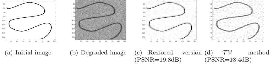
FIG. 16. Comparison of the restoration (5.3) ( \beta = 1 ) with the \mathcal{TV} model for a Gaussian blurred ( \sigma = 1.5 ) and Gaussian noisy (PSNR=15.7dB) synthetic image
