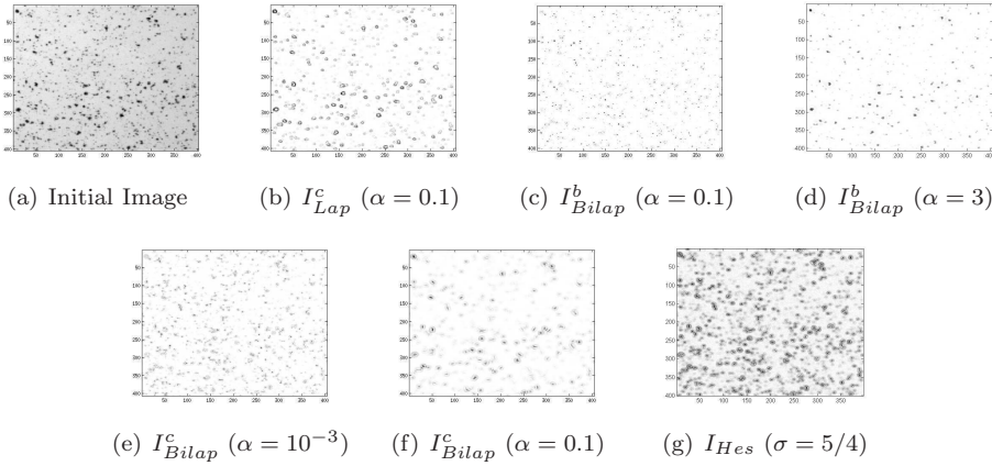
FIG. 11. Comparison of I_{Lap}^c (5.1), I_{Bilap}^b (4.3a), I_{Bilap}^c (4.3b) and I_{hes}^p (6.1) on a real image containing cells of different sizes
