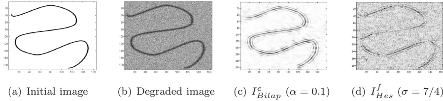
FIG. 14. Comparison of I_{Bilap}^c (4.3b) and I_{Hes}^f (6.1) for a Gaussian blurred ( \sigma = 2.1 ) and noisy (PSNR=15.7dB) image
