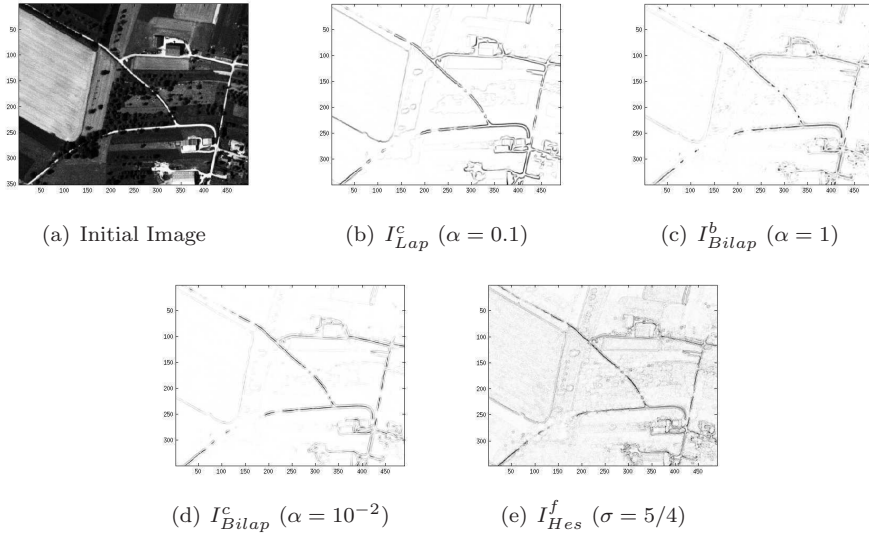
FIG. 6. Comparison of I_{Bilap}^b (4.3a), I_{Bilap}^c (4.3b), I_{Lap}^c (5.1) and I_{Hes}^f (6.1) on a real image
