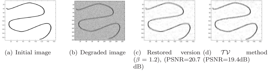
FIG. 17. Comparison of the restoration (5.3) with the \mathcal{TV} model for a synthetic image blurred by a convolution of type motion ( \theta = 90^\circ , length=7) and noised by a Gaussian noise (PSNR=15.7dB)
