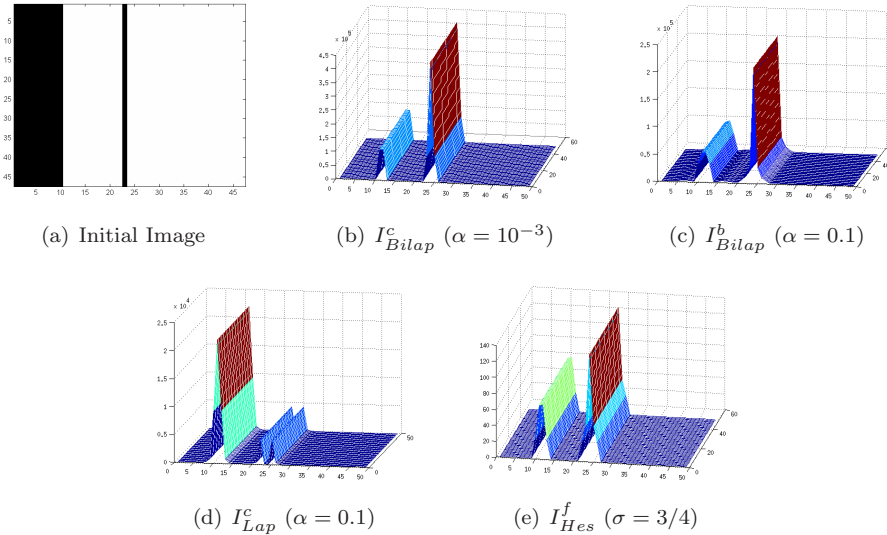
FIG. 5. Visualization of I_{Bilap}^b (4.3a), I_{Bilap}^c (4.3b), I_{Lap}^c (5.1) and I_{Hes}^f (6.1) on an edge and a filament on a synthetic image
