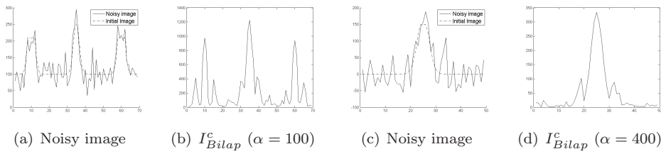
FIG. 25. A 1D cut ( y = y_c ) and ( z = z_c ) of I_{Bilap}^c (11.1) for two Gaussian noisy images (PSNR=16dB).
