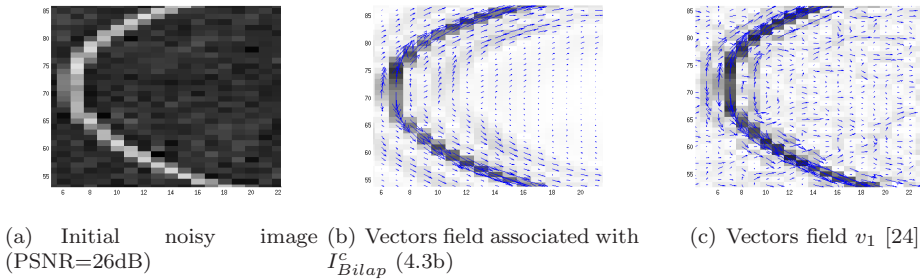
FIG. 9. The tangent vectors field given by (4.3b) compared to the vectors field v_1 [24]. For (b) the length of the vectors is proportional to I_{Bilap}^c and for (c) it is proportional to I_{Hes}^f (6.1).
