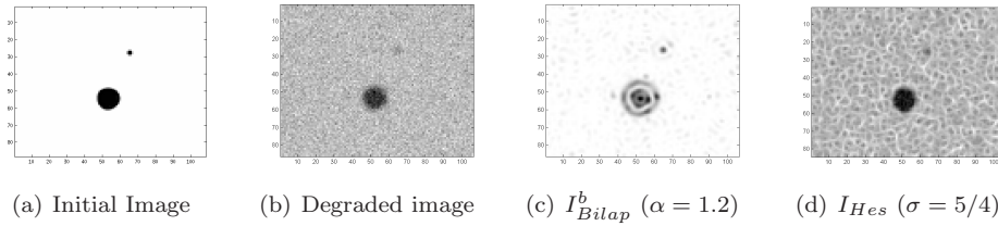
FIG. 21. Points detection by the topological indicator I_{Bilap}^b (4.3a) and the indicator I_{Hes} (6.1) on a synthetic image blurred by a Gaussian convolution ( \sigma = 1.5 ) and noised by a Gaussian noise (PSNR=15.7dB)
