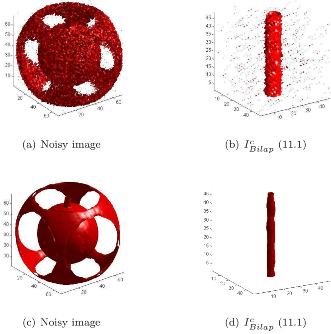
FIG. 23. Isosurfaces of I_{Bilap}^c (11.1) for two Gaussian noisy images (PSNR=16dB)
