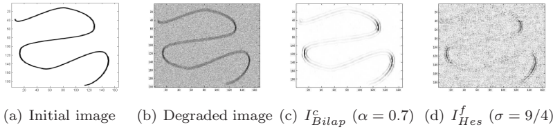
FIG. 15. Comparison of I_{Bilap}^c (4.3b) and I_{Hes}^f (6.1) for a motion blurred ( \theta = 90^\circ , length=7) and noisy image (PSNR=15.7dB)
