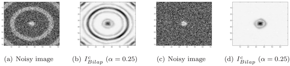
FIG. 24. A 2D cut ( z = z_c ) of I_{Bilap}^c (11.1) for two Gaussian noisy images (PSNR=16dB).
