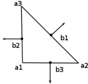
FIG. 3. The quadratic Morley finite element geometry
