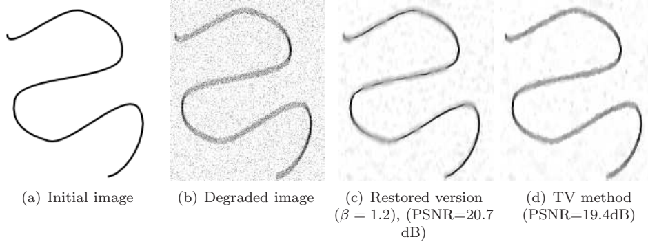
FIG. 17. Comparison of the restoration (5.3) with the TV model for a synthetic image blurred by a convolution of type motion ( \theta = 90^\circ , length=7) and noised by a Gaussian noise (PSNR=15.7dB)
