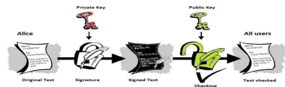
Figure 4: Digital Signature.
