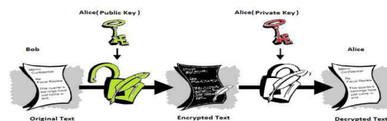
Figure 3: Encryption and Decryption with an Asymmetric Key.
