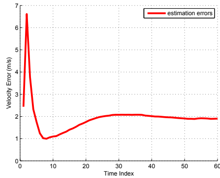
Figure 9: Velocity estimate errors for 100 Monte Carlo trials
