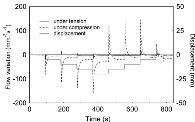
Fig. 6. Comparison of the flow patterns along the side under tension and the side under compression of a branch of Carpinus betulus during bending tests. Initial values of water flow are subtracted from the measured values.
