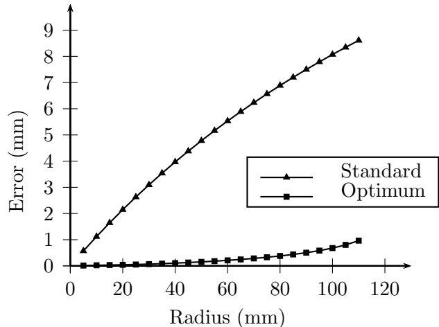
Figure 6: Error curves for any ruled surface
