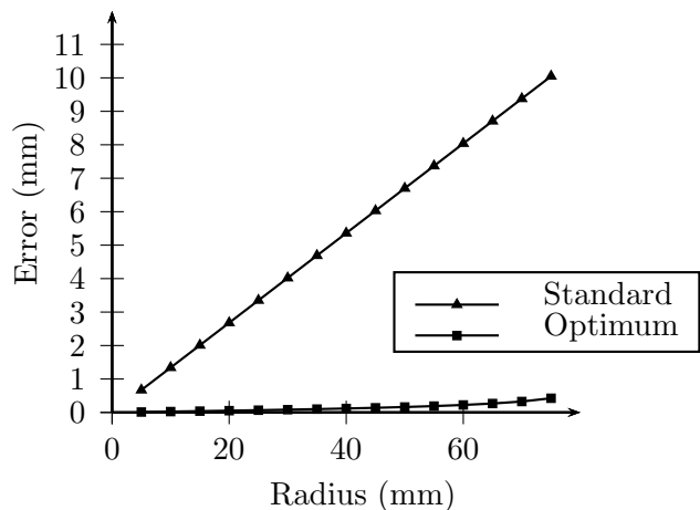
Figure 7: Error curves for a hyperbolic paraboloid ( \alpha = 30^\circ , h_p = 80mm )
