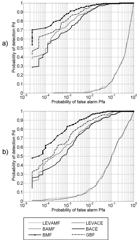
Fig. 4. ROC curves describing the detection of galvanized metal in: a) pure water ( H = 55 m, \text{SNR} = 5.6 dB); b) turbid water ( H = 14 m, C_\varphi = 0.7 \mu\text{g}\cdot\text{L}^{-1} , C_{CDOM} = 0.08 \text{ m}^{-1} , C_{NAP} = 2.8 \text{ mg}\cdot\text{L}^{-1} , \text{SNR} = 9.9 dB).
