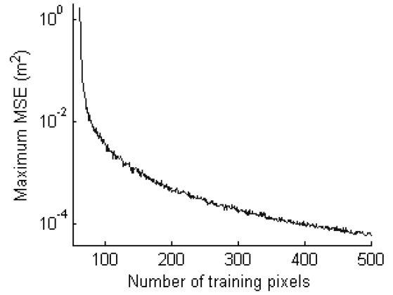
Fig. 7. Maximum MSE of the difference between the depth estimate under hypothesis H_0 or H_1 , and the depth estimate \hat{H} calculated only on training data, as a function of N ( H = 10 m, turbid water).
