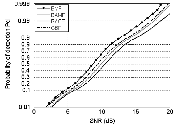
Fig. 5. Probability of detecting galvanized metal as a function of SNR ( H = 14 m, C_\varphi = 0.7 \mu\text{g}\cdot\text{L}^{-1} , C_{CDOM} = 0.08 \text{ m}^{-1} , C_{NAP} = 2.8 \text{ mg}\cdot\text{L}^{-1} ). The PFA is fixed at 10^{-4} .
