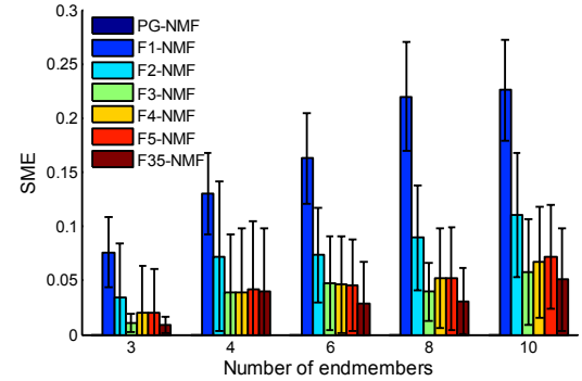
Fig. 2. Algorithm performances for different values of J .
