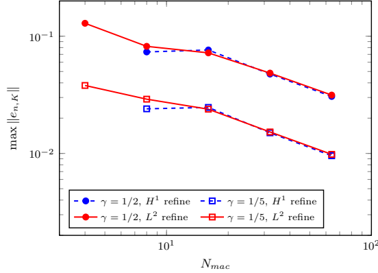
Figure 4: Tests for linearization error e_{n,K} , see (31), for test problem of Section 6.1 using tensor a^\varepsilon with \gamma = 1/2 (circle marks) and \gamma = 1/5 (square marks). Error term measured by \max \|e_{n,K}\| as a function of N_{mac} . Constant number of time steps N = 1024 . Macro and micro meshes according to Table 1 using H^1 refinement (dashed line) and L^2 refinement (solid line), respectively.
