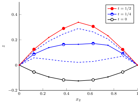
(a) Linearized scheme. N_{mac} = N_{mic} = N = 8 .
