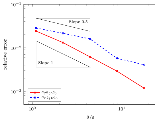
Figure 6: Degenerated parabolic multiscale problem of Section 6.2. Effect of sampling domain size \delta for linearized multiscale method (15) using Dirichlet coupling W(K_\delta) = H_0^1(K_\delta) . Sampling domain size \delta taken as \delta = 2^k \log(3)\varepsilon for k = 0, \dots, 4 . Temporal and spatial macro and micro discretization errors kept constant. Comparison to solution obtained by the linearized multiscale scheme (15) with optimal periodic coupling.
