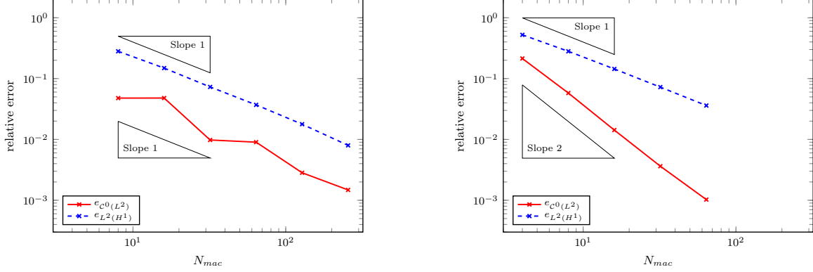
(a) H^1 refinement strategy. Macro and micro meshes with N_{mac} = 8, 16, 32, 64, 128, 256 and N_{mic} = 3, 4, 6, 8, 11, 16 .
