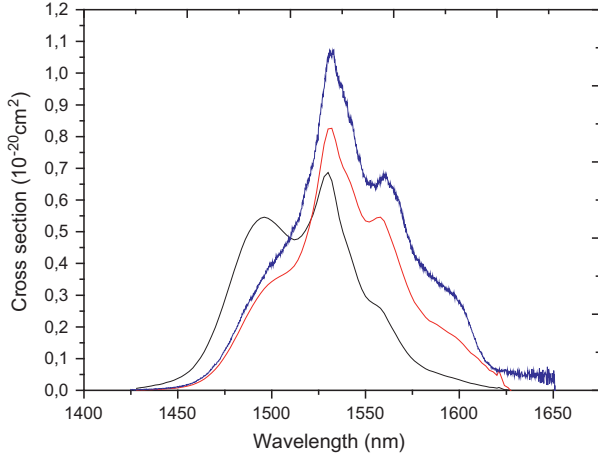
Fig. 3. {}^4{}_{13/2} \rightarrow {}^4{}_{15/2} absorption cross section (black curve) and {}^4{}_{13/2} \rightarrow {}^4{}_{15/2} emission cross section by M-C (red curve) and F-L (blue curve) formulas in the 0.5 mol% \text{Er}_2\text{O}_3 -doped SWNB glass. (For interpretation of the references to colour in this figure legend, the reader is referred to the web version of this article.)
