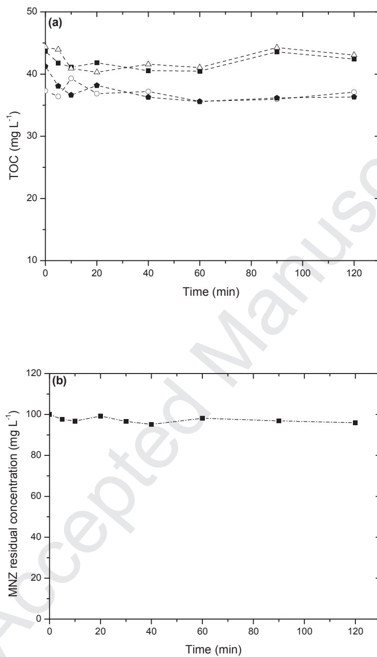
Fig. 5. Time-courses of the TOC values (a) and residual MNZ concentrations (b) during biosorption on activated sludge ( 0.5 \text{ g L}^{-1} ) of MNZ ( 100 \text{ mg L}^{-1} ) (---■---), and MNZ solutions electrolyzed in the absence (---○---) and in the presence of 10 \text{ mg L}^{-1} (---△---) and 20 \text{ mg L}^{-1} (---●---) of (\text{C}_5\text{H}_5)_2\text{TiCl}_2 .
