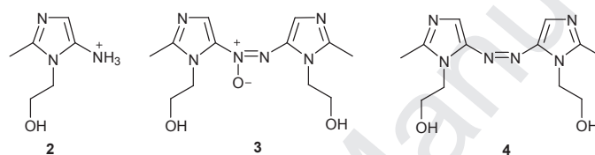
Scheme 1: Chemical structures of identified degradation by-products.
