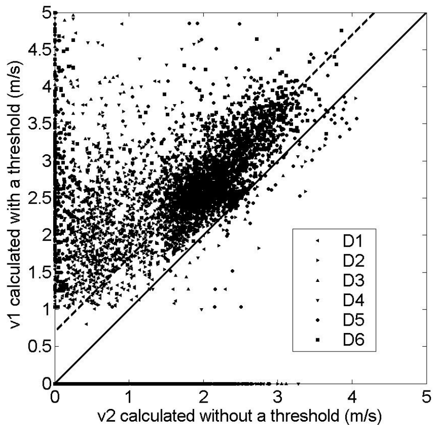
Figure 3: Comparison of calculated velocities with ( v_1 ) or without ( v_2 ) the use of a threshold level on gray scale images to detect tracers only. Line represents equality between v_1 and v_2 , and dashed line stands for a 0.7 m/s interval.
