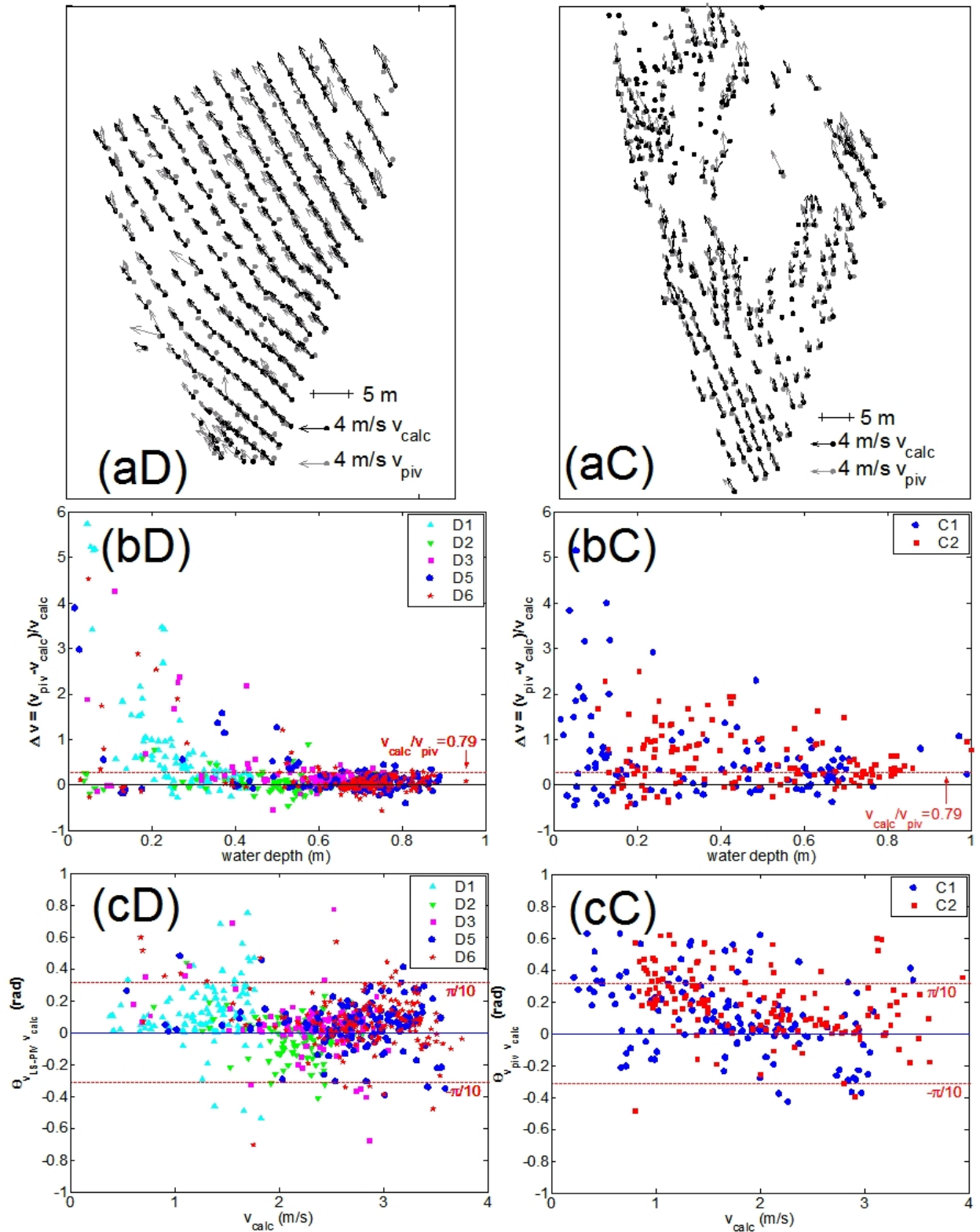
Figure 6: Comparison between LS-PIV velocity measurements ( v_{\text{piv}} ) and 2Dh numerical calculations ( v_{\text{calc}} ) on SITE D and SITE C: (a) velocity fields, (b) intensity comparison, (c) direction comparison.
