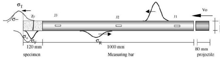
Figure 9: Principle of a dynamics tensile test by spalling, after [53].
