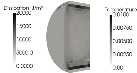
Figure 17: Volumic intrinsic dissipation for a quasi-static brazilian test, cross section
