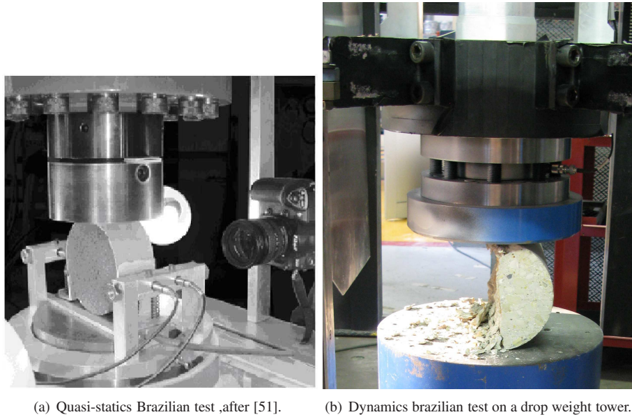
Figure 14: Experimental set-up for a brazilian test.
