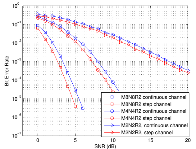
Fig. 6. Performances of differential space-time schemes with R = 2 bps/Hz over different channel models.
