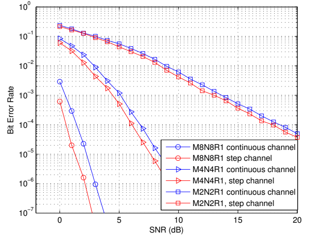
Fig. 5. Performances of differential space-time schemes with R = 1 bps/Hz over different channel models.
