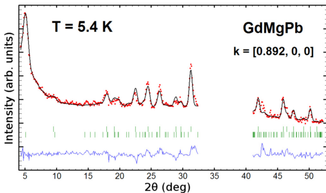
FIG. 11. (Color online) Refinement of the neutron powder diffraction pattern of GdMgPb recorded at 5.4 K with \lambda = 1.3286 \text{ \AA} . The top row of Bragg markers corresponds to the nuclear contribution and the bottom row corresponds to the magnetic contribution.
