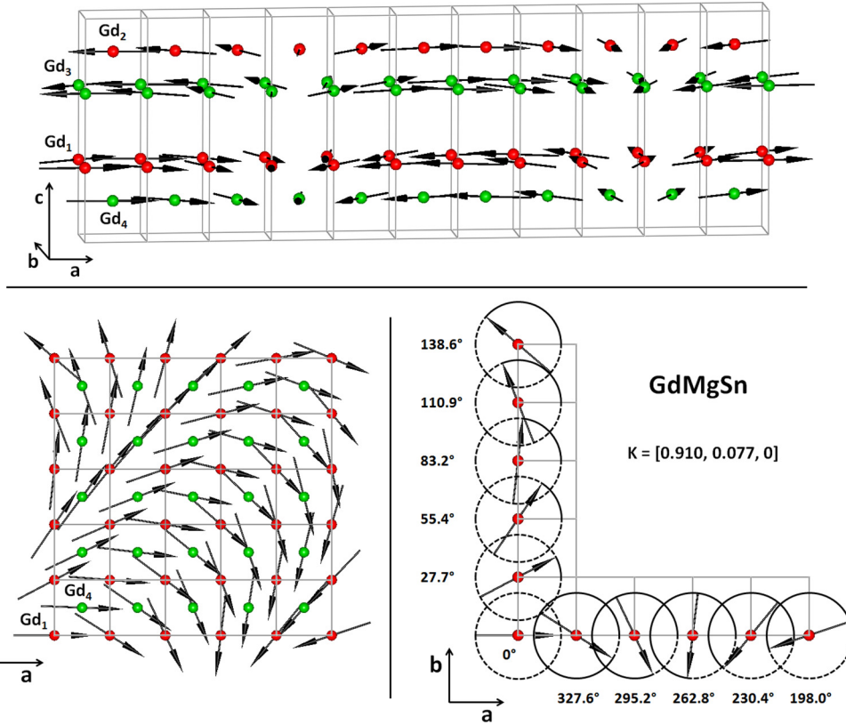
FIG. 10. (Color online) The cycloidal magnetic structure of GdMgSn at 5.4 K. For clarity, we have omitted the nonmagnetic Mg and Sn atoms.
