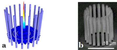
Fig. 1. Cylindrical photon cages : (a) electrical field map, (b) SEM image.
