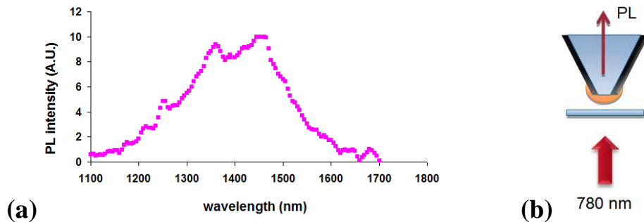
Fig. 2. Active NSOM probe : (a) photoluminescence (PL) spectrum (b) mode collection setup.
