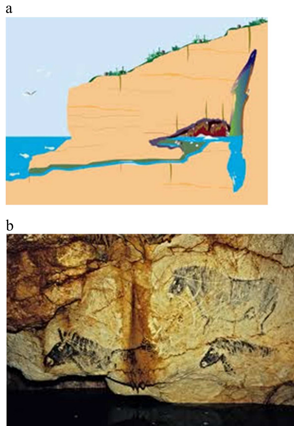
Figure 1. (a) Schematic view of the Cosquer cave (Marseille, France) under present-day sea level. (b) Prehistoric horse paintings (dated 18 500 years BP) in the partially submerged main chamber of the Cosquer Cave. Courtesy of V Feruglio and J Clottes
