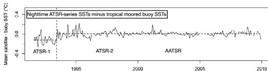
FIG. 4. An example assessment of stability of an SST dataset, adapted from Merchant et al. (2012). The figure shows a time series of monthly mean comparisons between nighttime satellite SSTs from ATSRs with matched SSTs measured in situ from tropical moored buoys. The early data are seen to be less stable, with a step change detected around 1993 (dashed lines). For 1995–2010, the 95% confidence interval for the stability of the satellite SST data are estimated to be -0.0018 to 0.0019 K yr -1 , which represents an uncertainty that should be accounted for in interpreting any trends in the satellite SST dataset.
