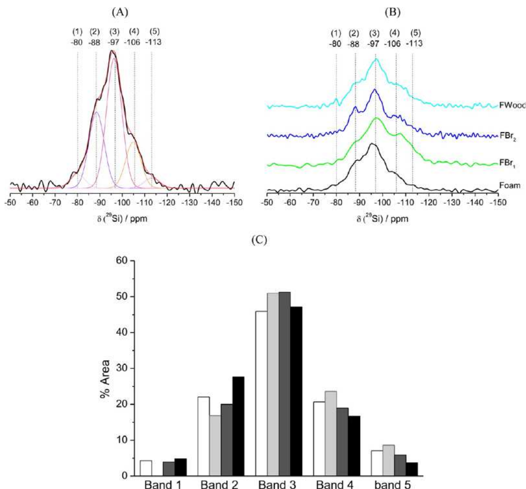
Figure 3. ^{29}\text{Si} MAS NMR results: (A) deconvoluted spectra in the case of FD S 100 (foam); (B) experimental data for FD S 100 W cod, FD S 100 B 1 , FD S 100 B 2 , and FD S 100 ; and (C) percentage of the area of each contribution determined from deconvoluted spectra for (white) FD S 100 W cod, (light gray) FD S 100 B 1 , (dark gray) FD S 100 B 2 , and (black) FD S 100 .
