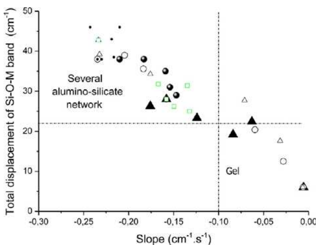
Figure 7. Evolution of the total displacement value versus the FTIR displacement slope value of Si-O-M band position for (filled triangle) FD S x M 5 100x , (open circle) S 400x M 5 100x , (large filled circle) S 400x FD S 100x , (open triangle) M 5x , (green box) FD S x , and (small filled circle) S 400x series.
