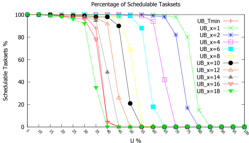
Figure 10: Schedulability by Varying x
