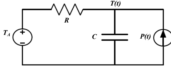
Figure 1: Thermal model
