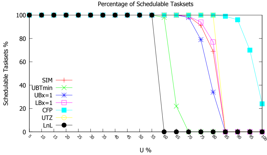
Figure 9: Percentage of Task sets that pass the test over U variation
