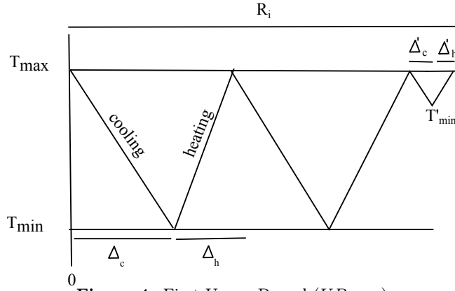
Figure 4: First Upper Bound ( UB_{T_{min}} )
