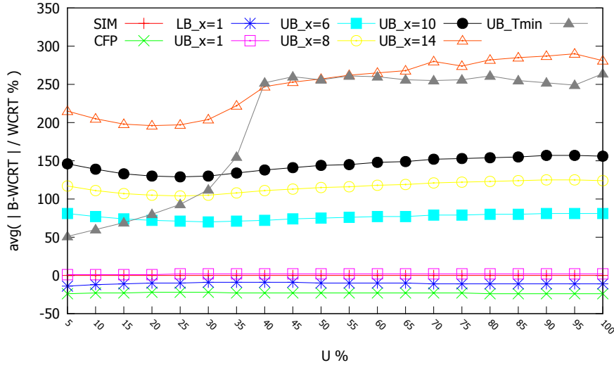
Figure 11: Bounds tightness over U variation
