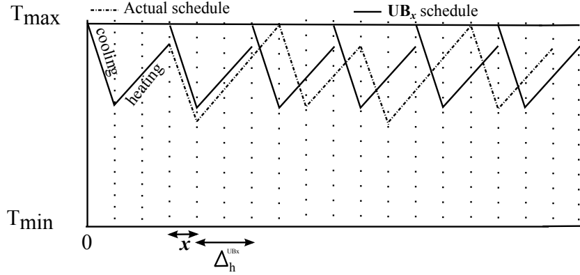
Figure 5: Parametric Upper Bound UB_x
