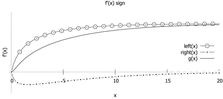
Figure 7: f'(x) 's sign
