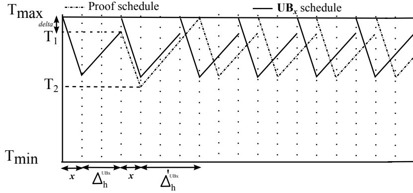
Figure 6: UB_x proof insight
