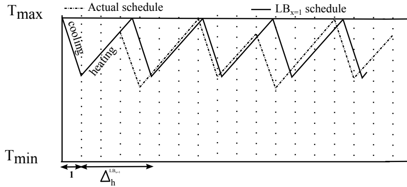
Figure 8: Lower Bound ( LB_{x=1} )
