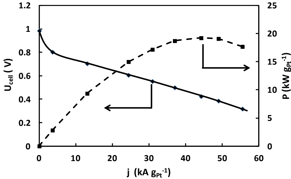
Figure 6. U_{\text{cell}} vs j and P vs j curves obtained at 70 °C with a membrane electrode assembly (MEA) consisting in a Nafion 212 membrane sandwiched between symmetrical 0.010 \text{mg}_{\text{Pt}}\text{cm}^{-2} Pt /CPL electrodes (flow rates of 350 \text{cm}^3 \text{min}^{-1} for \text{O}_2 and 500 \text{cm}^3 \text{min}^{-1} for \text{H}_2 ; T_{\text{O}_2} = 40 °C, T_{\text{H}_2} = 80 °C, P_{\text{O}_2} = 4 bar, P_{\text{H}_2} = 3 bar).
