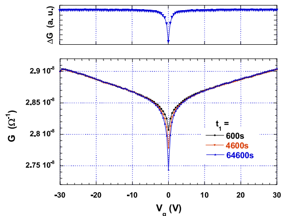
FIG. 3: Same data as in Figure 2 but on a larger V_g scale. Upper graph: difference in arbitrary units between two G(V_g) curves: one measured a few minutes after the cooling down and the other one about 20h later.
