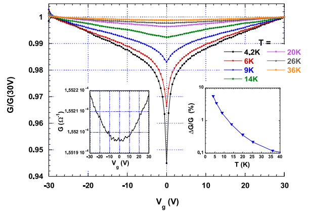
FIG. 5: Conductance dip measured at different T and normalized at V_g = 30V . The sample was first cooled down from 300K to 4.2K under V_{geq} = 0V and let at 4.2K for a few days before any T changes. The temperature was then increased, by steps, from 4.2 to 36K and kept constant during 1h before a G(V_g) scan (no significant changes in the amplitude are observed beyond this time scale). Left-side insert : G(V_g) scan at 300K (a linear background has been subtracted)[21]. Right-side insert: relative conductance difference between V_g = 30V and 0V as a function of T.
