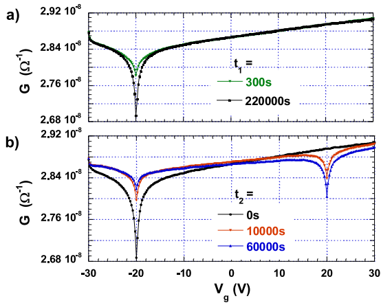
FIG. 4: (a) G(V_g) curves measured as a function of the time t_1 elapsed since the cooling down from 300K to 4.2K ( V_{geq} = -20V ). (b) G(V_g) curves measured a time t_2 after a V_{geq} change from -20V to +20V.
