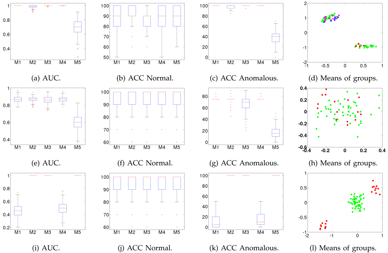
Fig. 7: Boxplots show the ACC and AUC statistics for group anomaly detection for three experiments, each row is a experiment. Marks on the x-axis of each boxplot represents the models: SMDDCCP (M1), SMDDDA (M2), SMDDDA with spherical normalization (M3), OCSMM (M4), and SVDD (M5). Also in the last column (Figures 7d, 7h, and 7l) plots the means of non-anomalous groups vs. the means of anomalous groups for the experiments considered.
