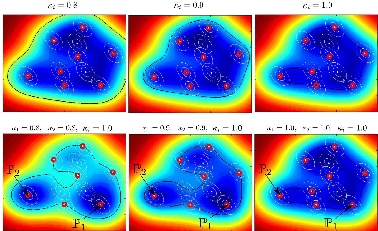
Fig. 5: The effect of different \kappa -values of Model M1 in the description of a dataset of probability measures.
