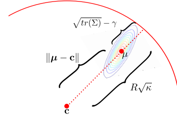
Fig. 3: Geometric interpretation of the deterministic constraints.
