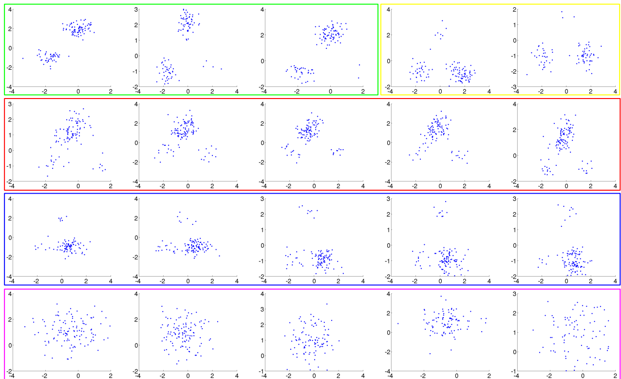
Fig. 6: Group anomaly detection dataset. Green and yellow boxes contains non-anomalous groups. Red, blue, and magenta boxes contains anomalous groups.
