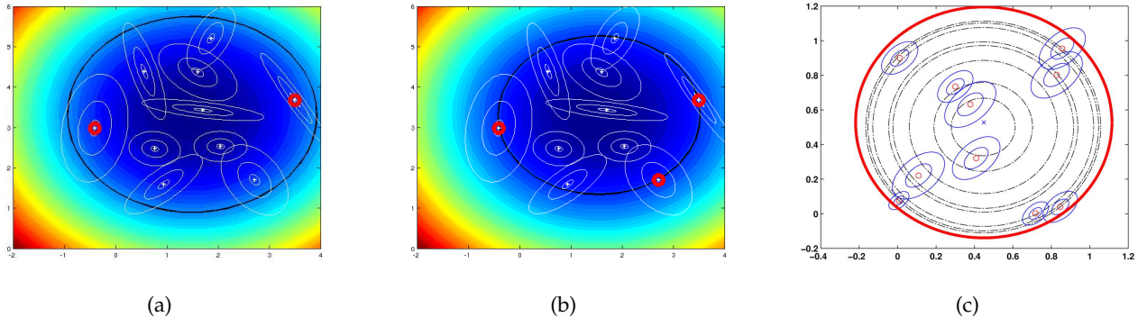
Fig. 4: Minimum enclosing balls from Models M1 and M2 with linear kernel for (14) and regularization parameter \lambda = 1 showed in (a) and (b). Minimum enclosing balls for several choices of \lambda for Model M5 (dashdot black circles) and a minimum enclosing ball from Model M5 with \lambda = 1 (red circle) showed in (c). Small Red points indicate support measures.
