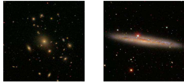
(a) A galaxy cluster
