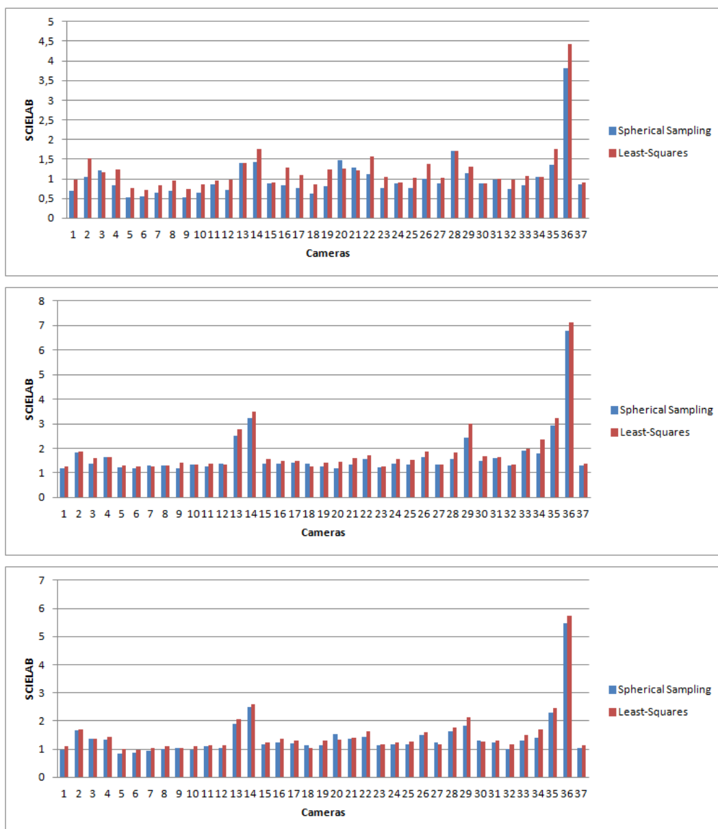
Figure 11. SCIELAB error for the different cameras computed as the mean for the different images. In blue: S-CIELAB error for spherical sampling. In red: error for the least-squares minimization. Top: First dataset. Middle: Second dataset. Bottom: Third dataset.
