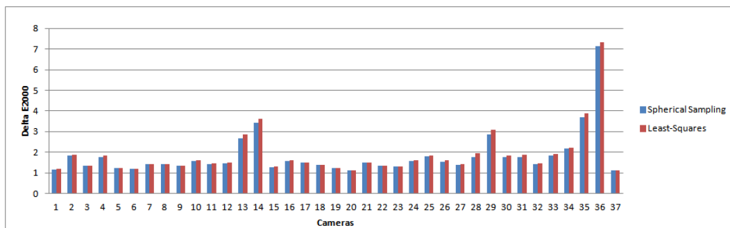
Figure 5. 98 per cent percentiles per camera for both the Spherical Sampling (blue) and the least-squares (red).
