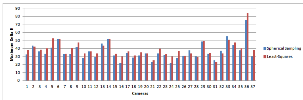
Figure 6. Maxima per camera for both the Spherical Sampling (blue) and the least-squares (red).
