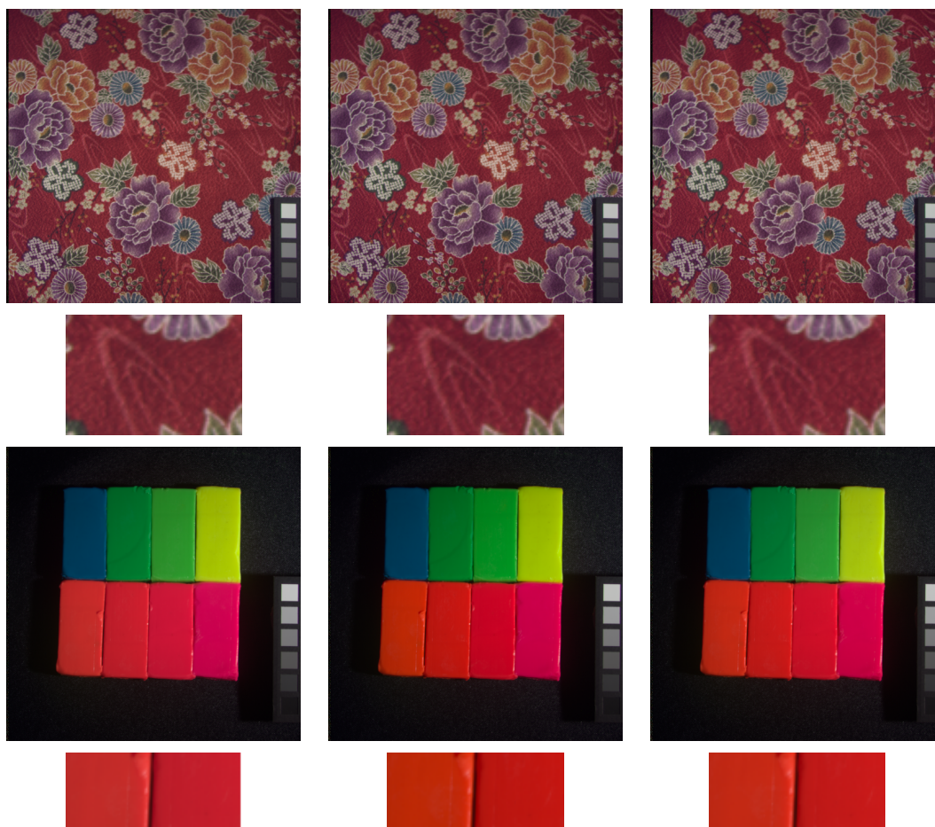
Figure 14. Qualitative evaluation of the approach versus matrix sampling. Top two rows: minimising the SCIELAB measure: full image (first row) and detail (second row). Last two rows: minimising the CID measure: full image (third row) and detail (last row). For each column the images are: Matrix sampling (left), original (centre), spherical sampling (right)
