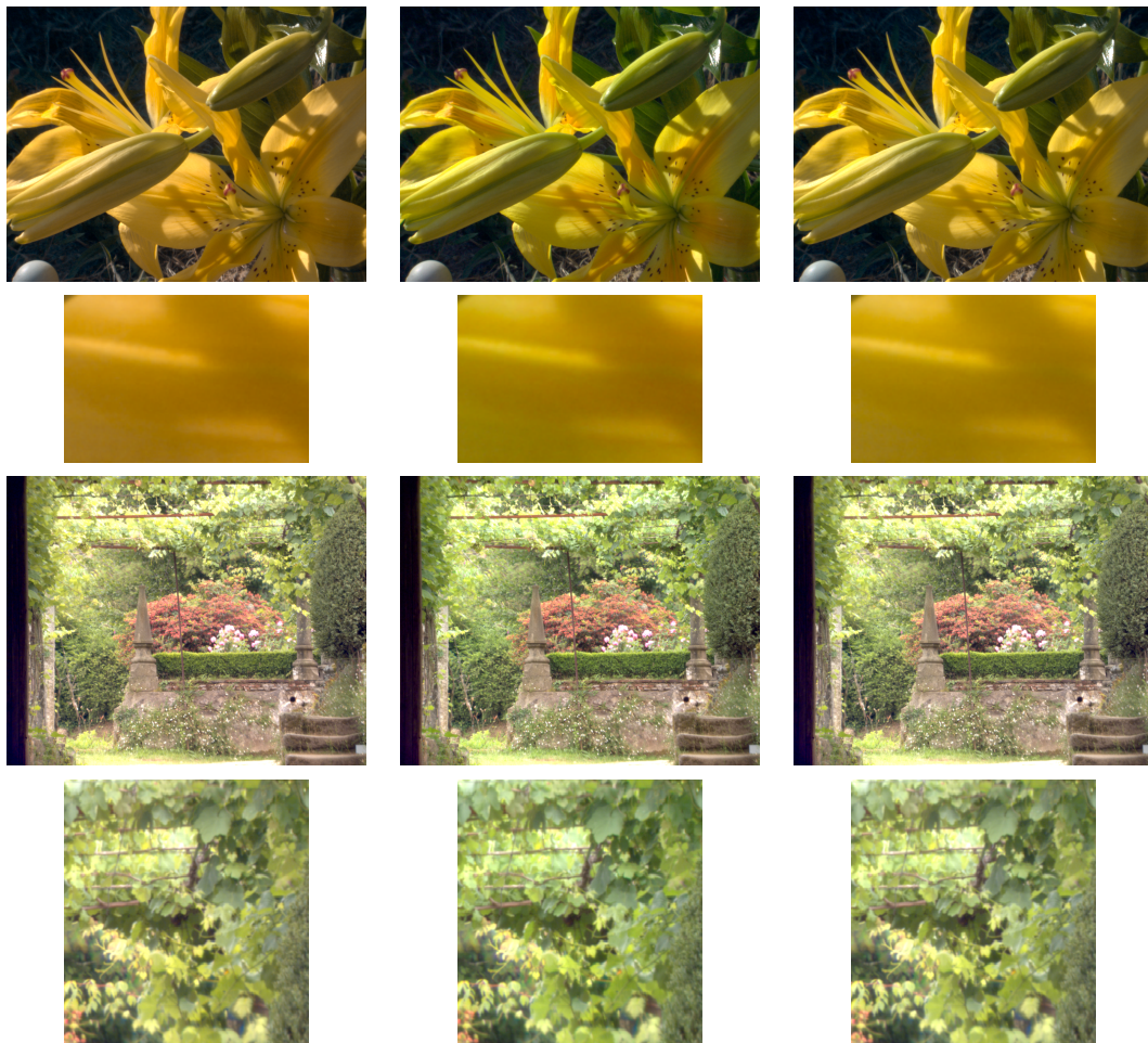
Figure 13. Qualitative evaluation of the approach. Top two rows: minimising the SCIELAB measure: full image (top column) and detail (second row); last two rows: minimising the CID measure: full image (third row) and detail (last row). For each column the images are: Original (left), least-squares (centre), spherical sampling (right)
