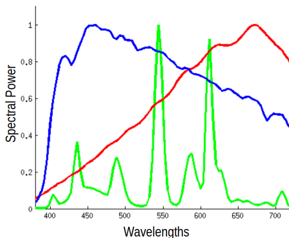
Figure 8. Spectral sensitivities of the three illuminants used in Experiment 1b.
