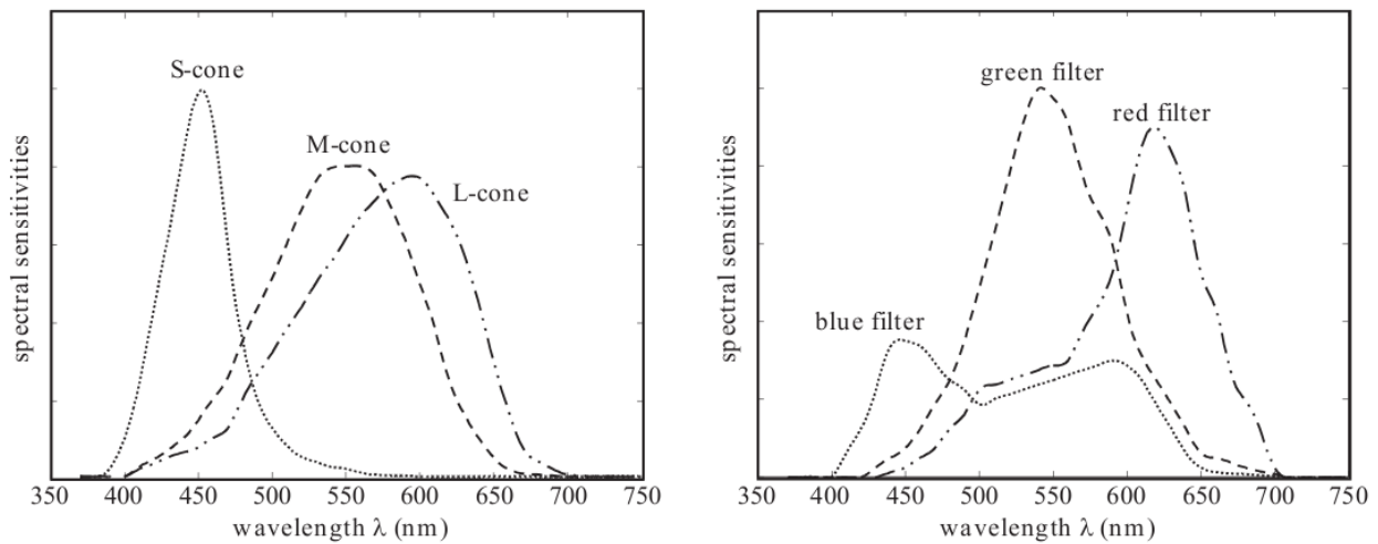
Figure 1. Spectral sensitivities of: (a) the three types of cones in a human eye, and (b) a typical digital camera. Images from [1].
