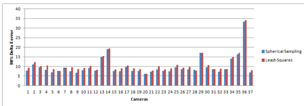
Figure 5. 98 per cent percentiles per camera for both the Spherical Sampling (blue) and the least-squares (red).
