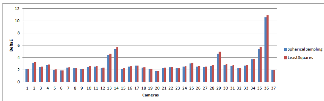
Figure 3. \Delta E error for the different cameras. In blue: \Delta E for spherical sampling. In red: error for the least-squares minimization.
