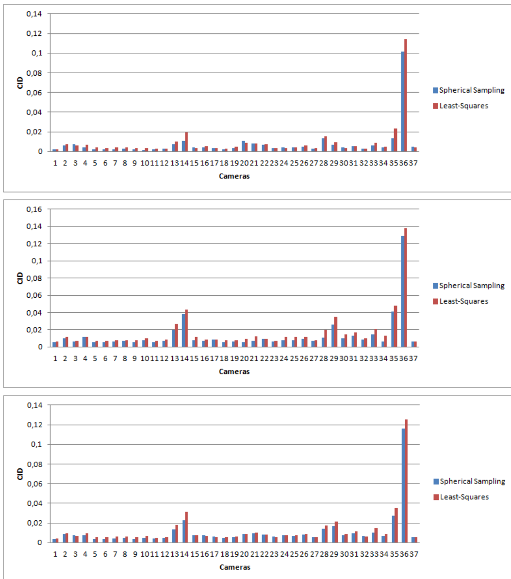
Figure 12. CID error for the different cameras computed as the mean for the different images. In blue: CID error for spherical sampling. In red: error for the least-squares minimization. Top: First dataset. Middle: Second dataset. Bottom: Third dataset.
