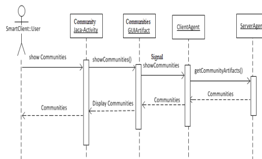
Figure 3. Interaction between ClientAgent and ServerAgent
