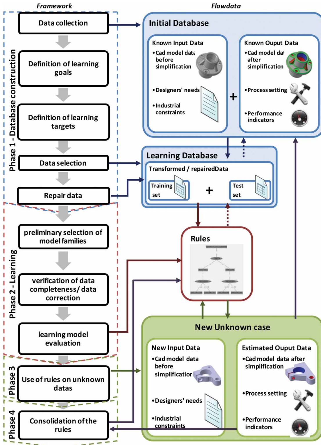
Fig. 3: Data flow and framework of the proposed approach.
