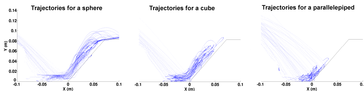
Fig. 4. The block trajectory in the embankment vicinity is strongly influenced by the rock shape
