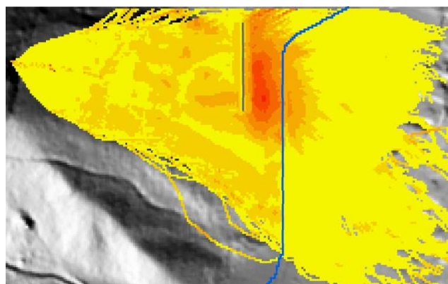
Fig. 1 3D rockfall simulation may result in abnormal block passing heights in the embankment vicinity
