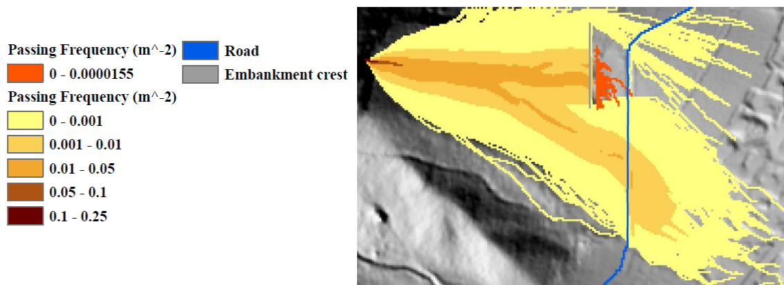
Fig. 3 Adopting a specific rebound model and coupling a high resolution DTM model in the embankment vicinity to a "normal" model at the site scale allows coping with the abnormal trajectories observed Fig. 1
