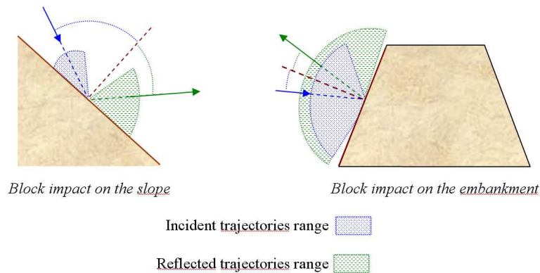
Fig. 2 Ranges of incident and reflected trajectories on the slope and on the embankment facing
