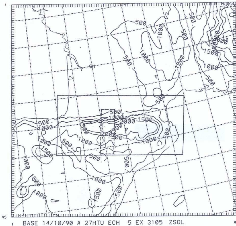
Fig. 20. Horizontal domains for the momentum budget computations with the outputs of the Péridot model. The smaller box is the validation box covering only the central transect. The larger box is well suited for an evaluation of the global effect of the mountain
