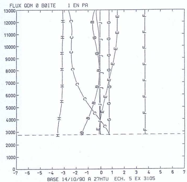
Fig. 22. Same as in Fig. 21, but on the larger box
