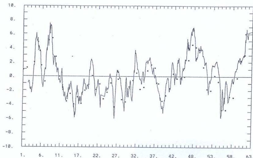
Fig. 4. The 2 months time series of the surface pressure drag computed from measurements of the CNRM portable network (continuous thin line). The SLP difference between Pau and Zaragoza is shown as symbols. The abscissa is in days, starting from 1 October 1990. The ordinate is to be understood as Pascals for the drag, and hPa for the SLP difference. (from Puech et al. , 1991)
