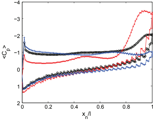
Fig. 5. Pressure coefficient C_p distribution along the airfoil extrados (upper curves) and intrados (lower curves) time-averaged in the range: \circ, 8 \leq tU_0/l \leq 13.6 ; \times, 8 \leq tU_0/l \leq 9.2 ; +, 9.2 \leq tU_0/l \leq 10.4 . Here, x_n is the distance from the airfoil nose.
