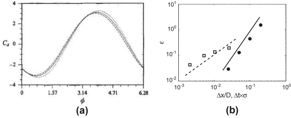
Fig. 7. (a) Time evolution of the drag coefficient C_D over an oscillation cycle: (---), present method; (—), pseudo-spectral method of Chang and Maxey [11]; (- - -), experiments of Odar and Hamilton [48]; (· · · · ·), analytical solution. Here \sigma t = \phi/2\pi . (b) Error computed from the maximum value of C_D at the end of the second cycle as a function of (●) spatial resolution and (□) time step. The reference value of C_D used for the spatial and temporal convergence analysis is the one obtained with ( \Delta x/D = 1.25 \times 10^{-2} ; \sigma \Delta t = 10^{-2} ) and ( \Delta x/D = 5 \times 10^{-2} ; \sigma \Delta t = 10^{-3} ), respectively. The dashed and solid lines indicate first- and second-order convergence, respectively.
