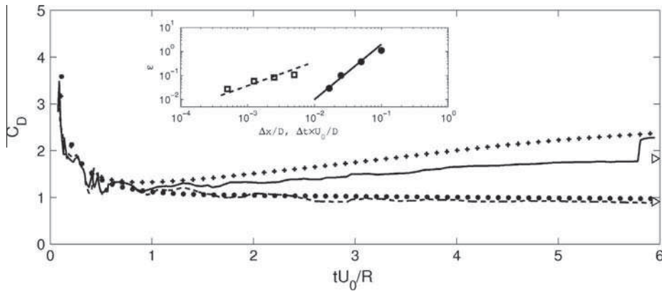
Fig. 17. Time evolution of the total drag coefficient C_D . Present method ( Re = 200, Sc \gg 1 ): + , Fr = 2 ; \bullet , Fr = 20 . Simulations from the boundary-fitted method of Torres et al. [61] ( Re = 200, Sc = 700 ): \text{---} , Fr = 2 ; \text{- - -} , Fr = \infty . The upper and lower triangles indicate the value of C_D reported in Fig. 13 of Hanazaki et al. [30] for Fr = 2 and Fr = 20 , respectively. Inset: Error computed from the value of C_D at time tU_0/R = 5 as a function of ( \bullet ) spatial resolution and ( \square ) time step. The reference value of C_D used for the spatial and temporal convergence analysis is the one obtained with (\Delta r/D = 1.25 \times 10^{-3}; \Delta t \times U_0/D = 2.5 \times 10^{-2}) and (\Delta r/D = 2.5 \times 10^{-2}; \Delta t \times U_0/D = 2.5 \times 10^{-4}) , respectively. The dashed and solid lines indicate first- and second-order convergence, respectively.
