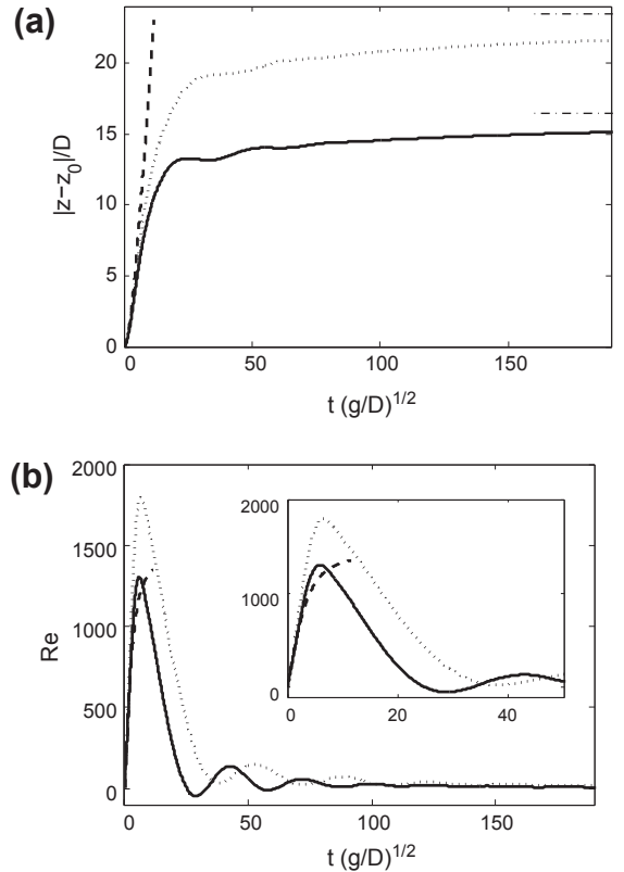
Fig. 19. Time evolution of (a) the vertical distance crossed by the sedimenting sphere and (b) local particle Reynolds number: (- - -) , Fr = \infty , \rho_p/\rho = 4.6 ; (\text{---}) , Fr = 4.3 , \rho_p/\rho = 4.6 ; (\cdots\cdots) , Fr = 4.3 , \rho_p/\rho = 6.1 . The dash-dotted lines indicate the location of the neutral buoyancy level for which \rho = \rho_p . Here, the simulation is three-dimensional.
