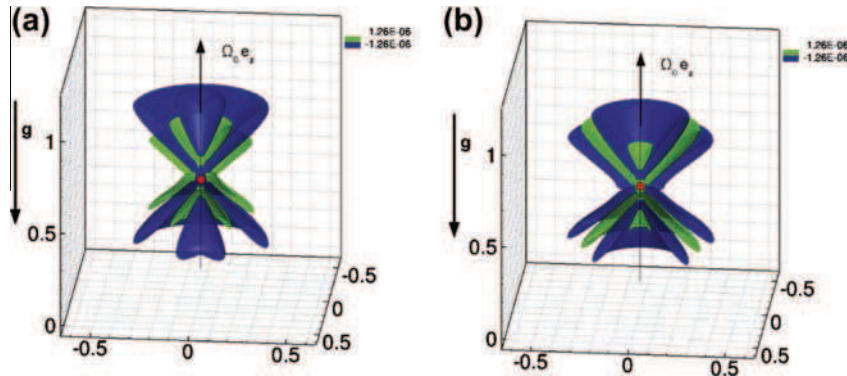
Fig. 11. Iso-surfaces of density fluctuations \delta\rho generated by an oscillating sphere in a rotating stratified fluid at (a) t\sigma/(2\pi) = 4.7 and (b) t\sigma/(2\pi) = 5.2 for Re = 100, Fr = 0.8, C = 0.316 and A_0/R = 1 . Iso-surfaces \delta\rho = \pm 1.26 \times 10^{-6} are plotted on half the computational domain in order to show the sphere location. Here, the simulation is three-dimensional.
