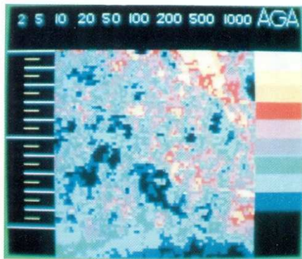
Figure 16 Small-scale variations of the infrared brightness temperatures over a 1 m 2 area of oats at Lubbon (site # 1) on June 16, 1986; the average temperature is 25 °C and the range is 3 K (provided by courtesy of M. P. Stoll and F. Nerry, GSTS, Strasbourg).
