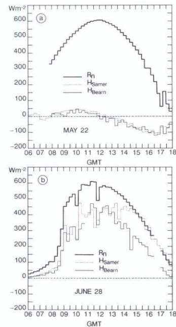
Figure 2 Comparison between surface fluxes H of sensible heat observed at Lubbon over oats (site # 1) by the SAMER (dotted line) and the BEARN (solid line) systems for (a) May 22 and (b) June 28, 1986. The heavy line shows the net radiative flux at the surface.
