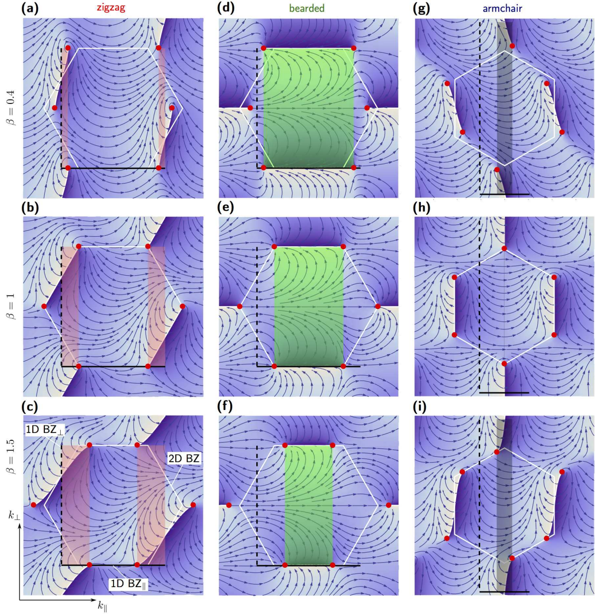
Figure 4. Stream and density plots of the phase \phi(k_{\parallel}, k_{\perp}) in reciprocal space, for the three edges (zigzag, bearded and armchair) and for various deformations (see the sketches in Figs 3 and 7). The first 2D (bulk) BZ is indicated by a white contour. The red dots are the positions of the Dirac points. The first 1D BZ associated to the ( \parallel ) and ( \perp ) directions are shown by solid and dashed black lines, respectively. For a given k_{\parallel} , the existence of edge states is related to the winding of the phase along the k_{\perp} direction in the BZ: there are edge states when the total rotation of the phase is 2\pi as seen in the shaded areas [ \mathcal{Z}(k_{\parallel}) = \pi ]. There are no edge states otherwise [ \mathcal{Z}(k_{\parallel}) = 0 ].
