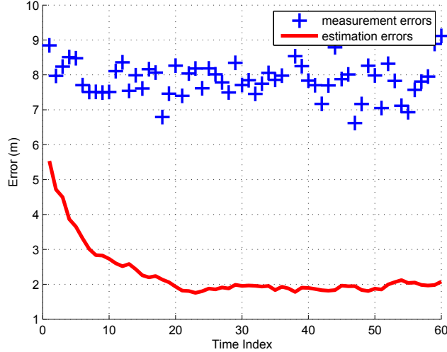
Figure 2: Estimation and measurement errors for 100 Monte Carlo trials
