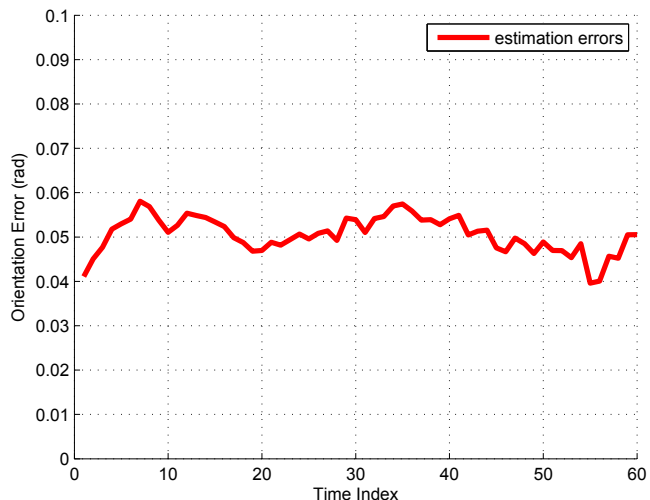
Figure 5: Orientation estimate errors for 100 Monte Carlo trials
