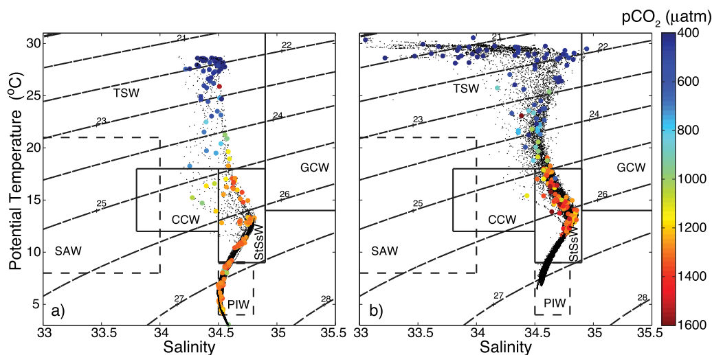
Figure 3. Potential temperature ( \theta ) and salinity diagram for cruises conducted in (a) November and (b) August 2010. \theta - S diagram for August shows the upper 500 m of the water column. The color bar indicates the p\text{CO}_2 value for each temperature and salinity measurement. TSW = Tropical Surface Water, StSsW = Subtropical Subsurface Water, GCW = Gulf of California Water, CCW = California Current Water, SAW = Subarctic Water, and PIW = Pacific Intermediate Water. Water masses were classified according to Fiedler and Talley [2006] and León-Chavez et al. [2010].
